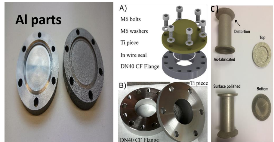
Al and Ti flanges and chambers
